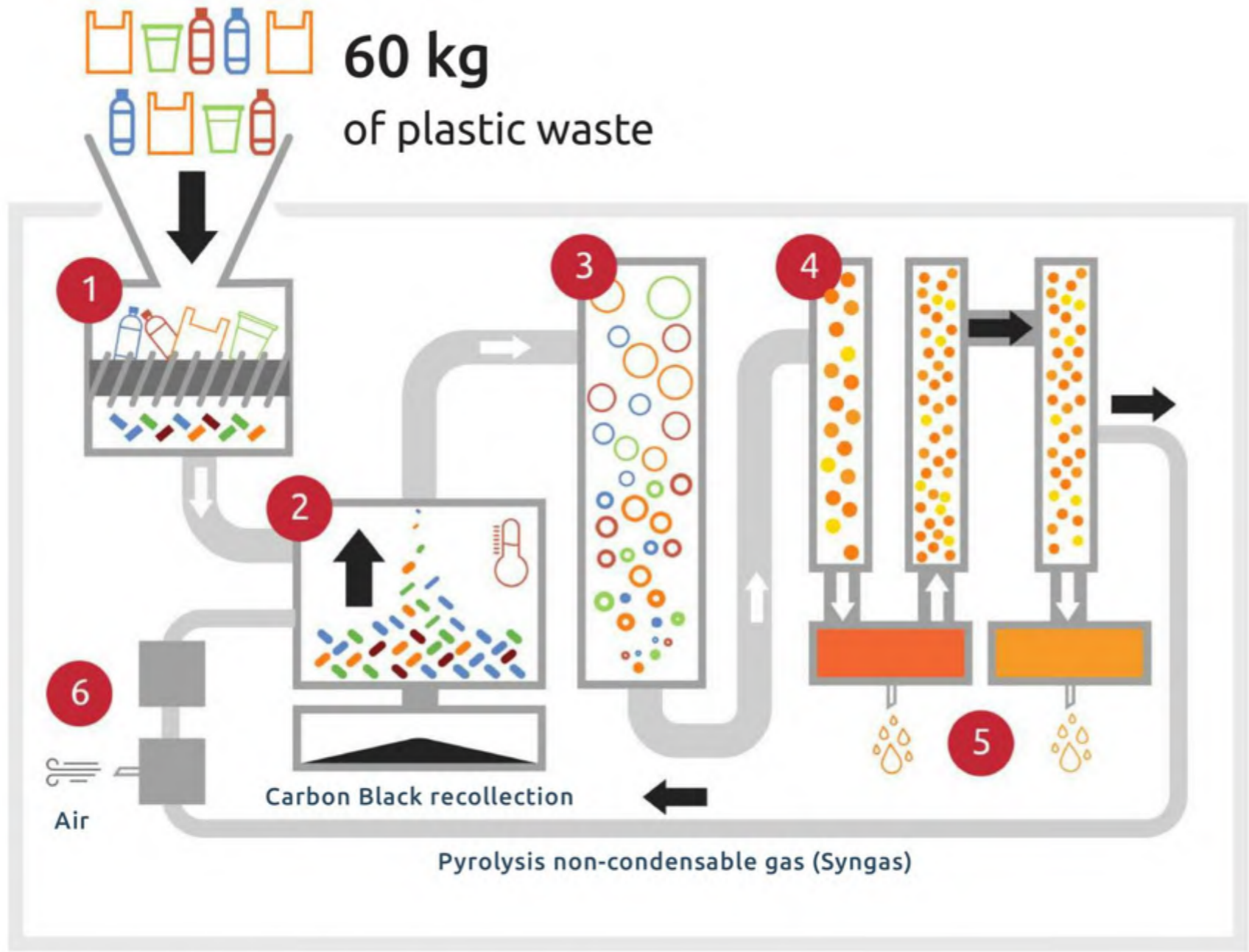
VIEW OF THE CONTAINERISED PYROLYSIS UNIT
